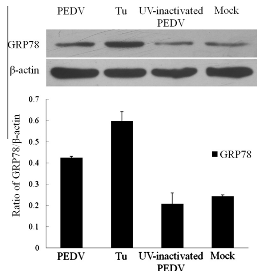
Fig. 4. PEDV replication is required for UPR induction. Vero cells were infected with UV-inactivated PEDV, PEDV (both MOI = 0.01) or treated with Tu (2 \mu g/ml). The cells were harvested at 24 h and Western blot was performed to determine UPR activation using anti-GRP78 antibody. \beta -Actin was used as a loading control.
